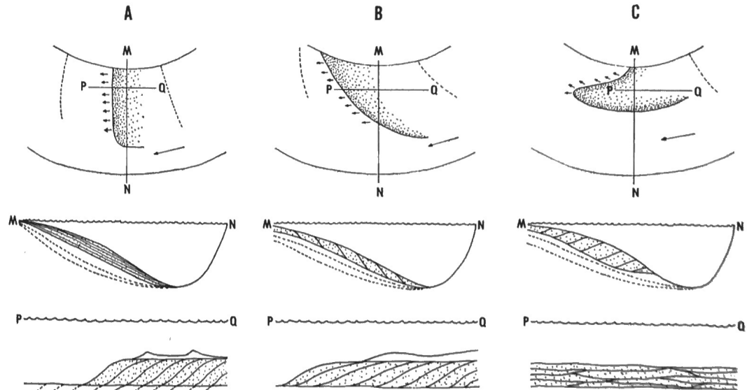
Figure 6. Idealized model illustrating the dependency of bedding geometry on bar-face orientation. Dashed lines indicate possible positions of preceding and succeeding bar faces.
