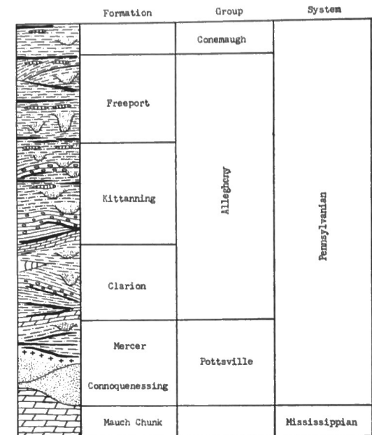
Figure 3. Generalized stratigraphic framework showing location of the Kittanning formation (Allegheny group) of Pennsylvanian Age.
